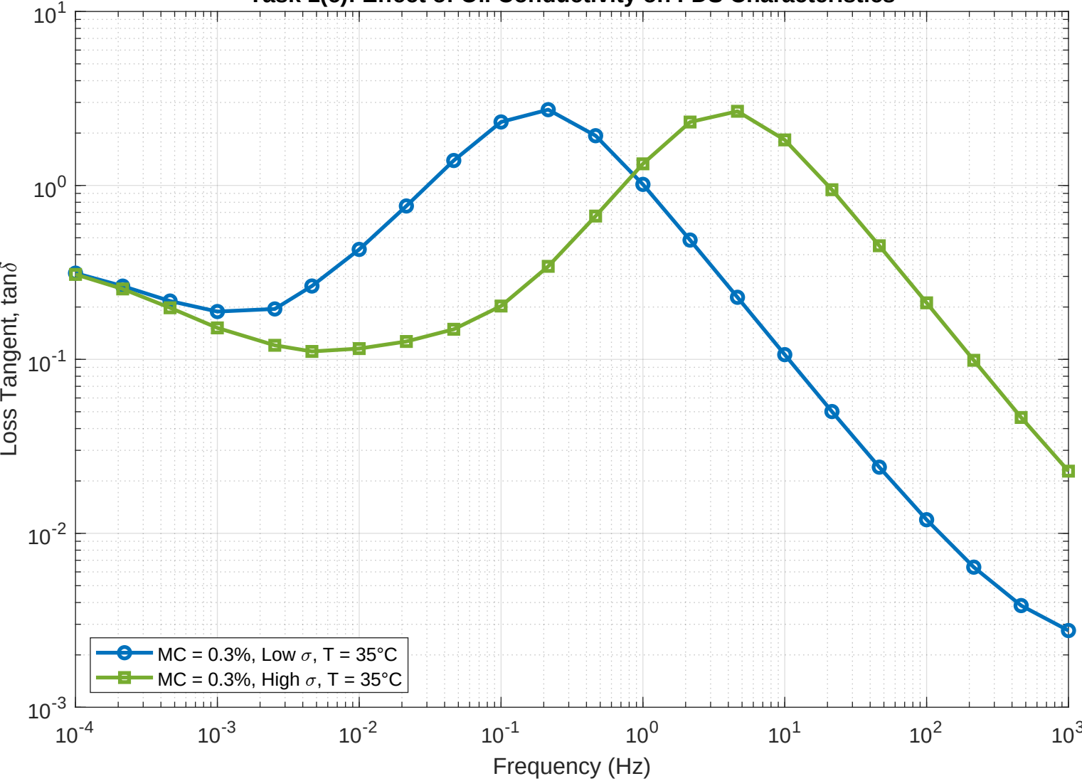
Task 1(c): Effect of Oil Conductivity on FDS Characteristics
